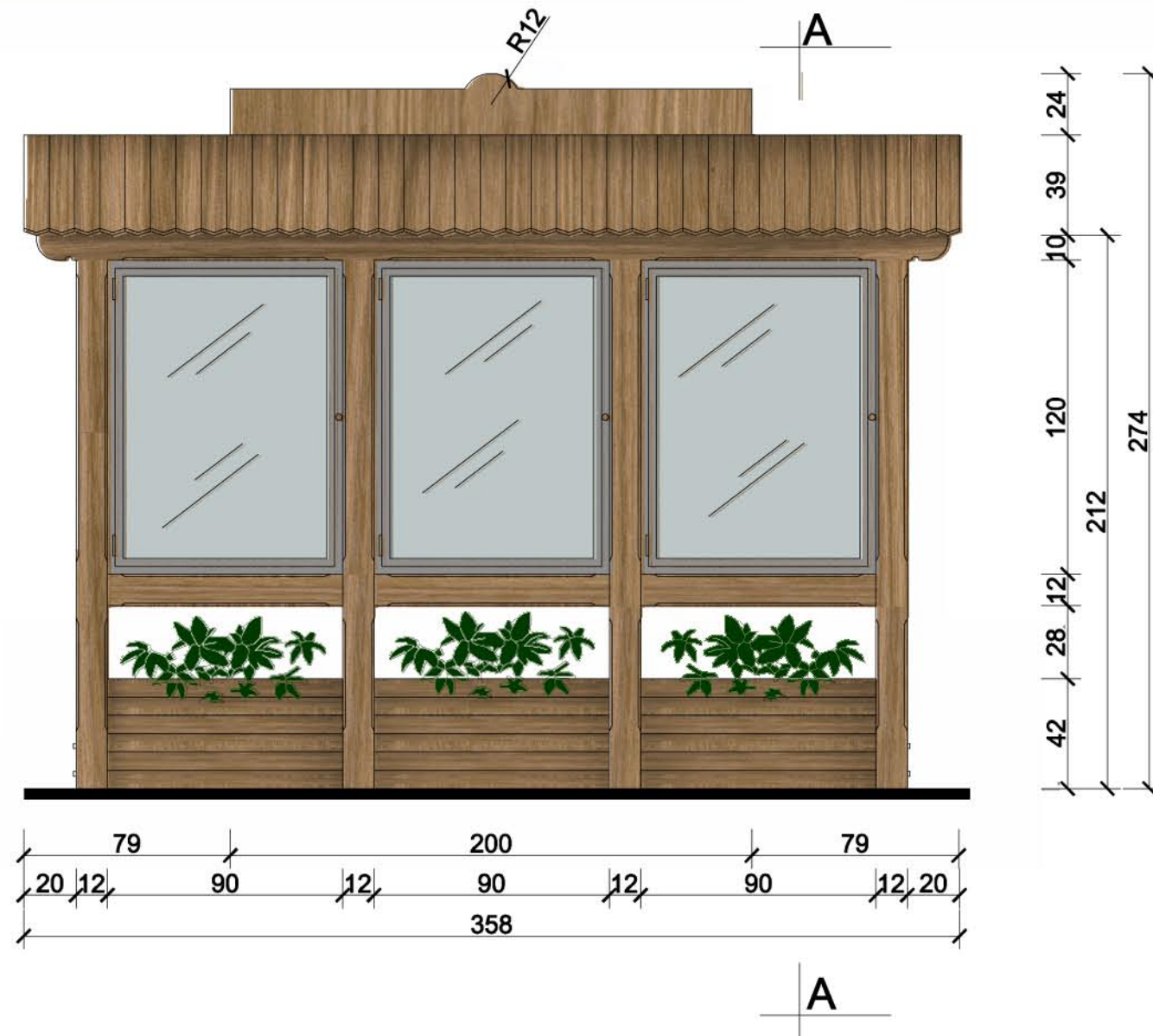
Element 1: 3D3, 3 pola, donice, 3 gabloty; skala 1:25
